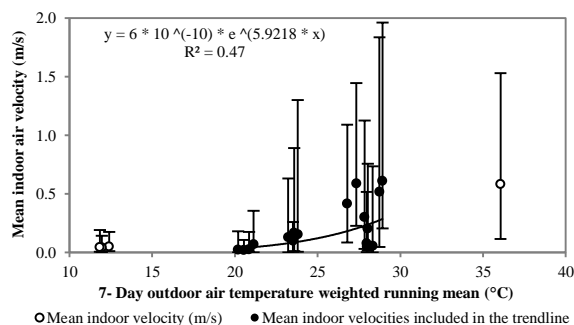
Figure 4 Variation in air velocity with outdoor air temperature
